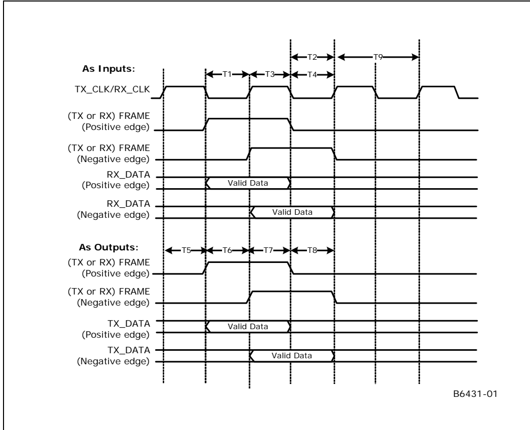
Figure 49-43.TDM, Serial Timings
