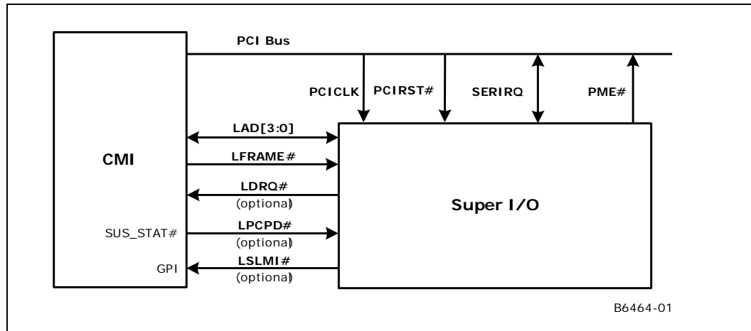
Figure 19-1. LPC Interface Diagram
